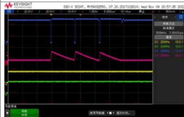
CH1: VIN CH2:VOUT CH3:SW CH4:IL Vin=20V Vout=20V Steady State waveform Iout =0A
