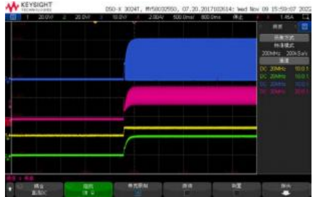
CH1: VIN CH2:VOUT CH3:SW CH4:IL Vin=8.4V Vout=20V Start up waveform through Vin, Iout =1A
