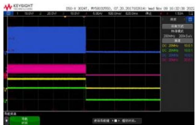
CH1: VIN CH2:VOUT CH3:SW CH4:IL Vin=8.4V Vout=20V Shut Down waveform through VIN, Iout =1A
