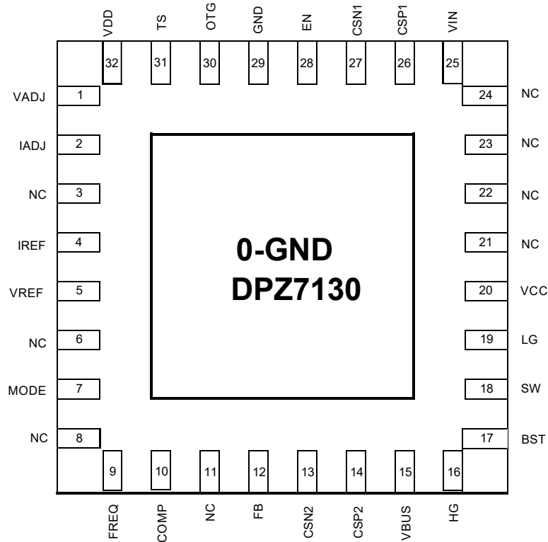
Fig. 2 Pin-Function (QFN4X4-32)
