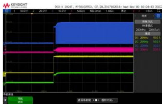
CH1: VIN CH2:VOUT CH3:SW CH4:IL Vin=16.8V Vout=20V Start up waveform through Vin, Iout =1A
