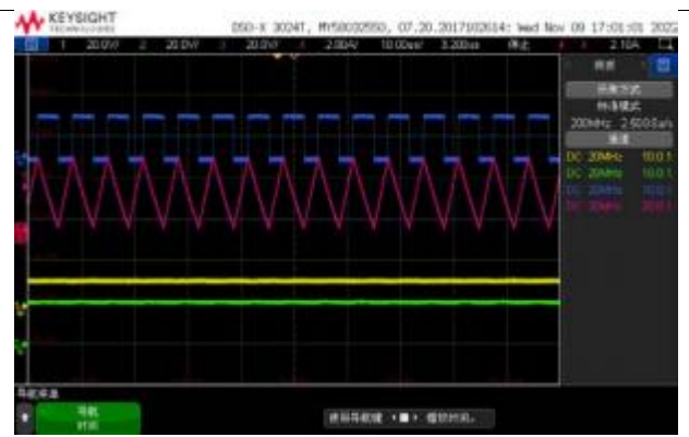
CH1: VIN CH2:VOUT CH3:SW CH4:IL Vin=12.6V Vout=20V Steady State waveform Iout =1A
