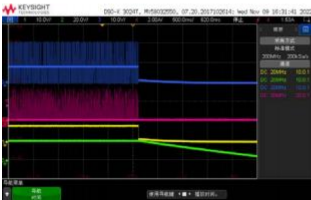
CH1: VIN CH2:VOUT CH3:SW CH4:IL Vin=8.4V Vout=20V Shut Down waveform through VIN, Iout =0A
