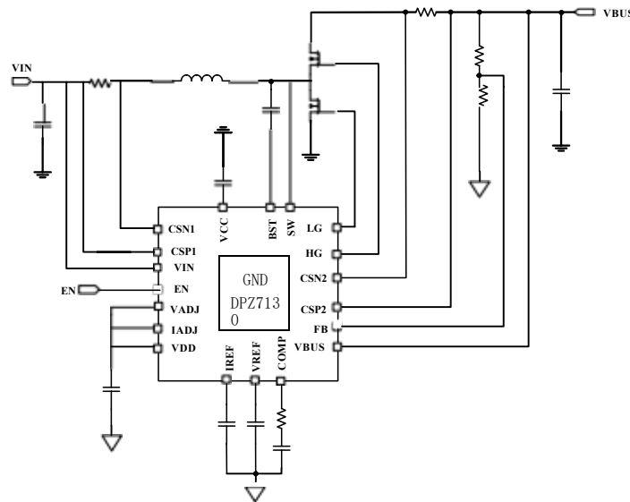
Fig. 1 Application Schematic
