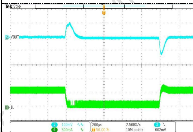
Load Step 0.1 to 0.6A, 1A/us Slew rate
