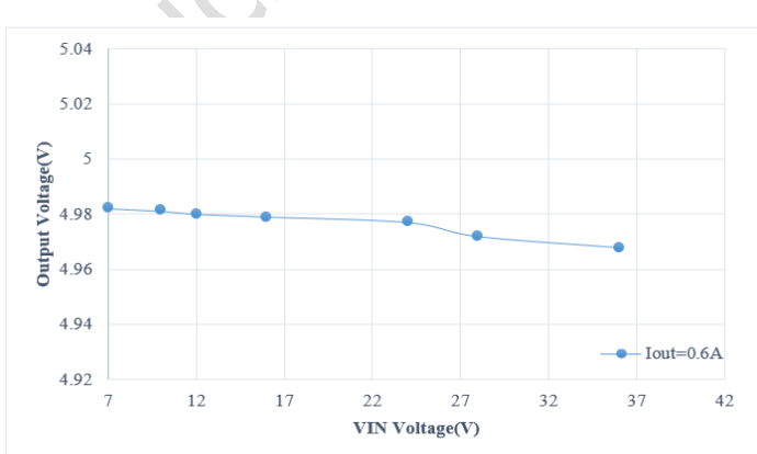
Figure4 Line Regulation Iout=0.6A
