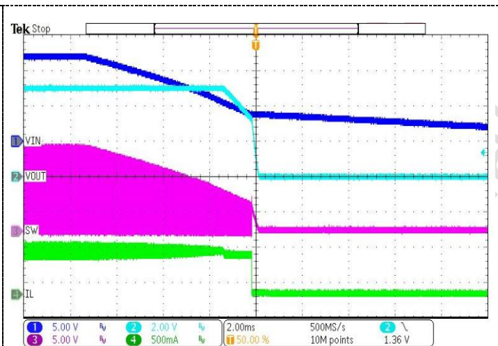
Figure8 ShutDown with Load
