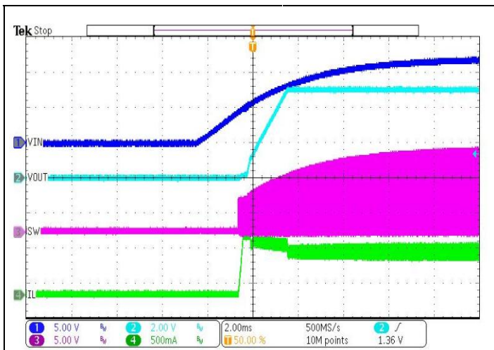
Figure7 VIN StartUp with Load
