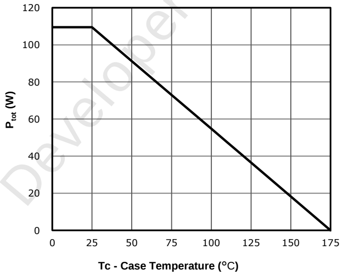
Figure 5. Power derating
