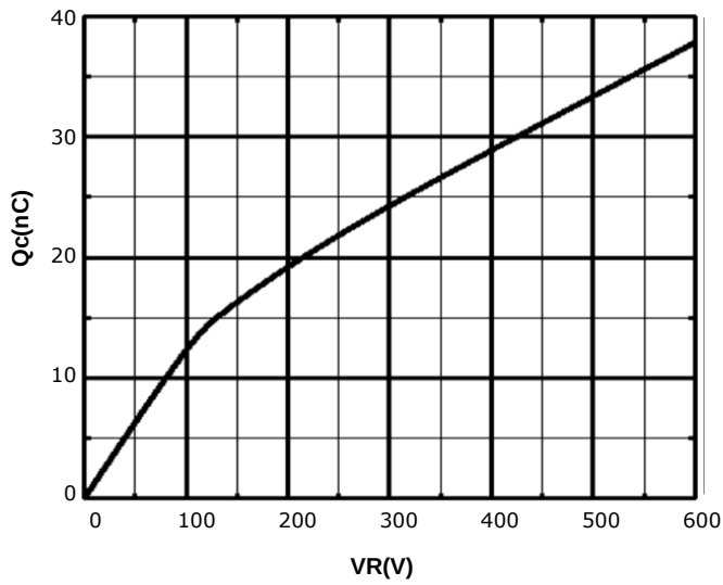
Figure 7. Total capacitance charge vs. reverse voltage
