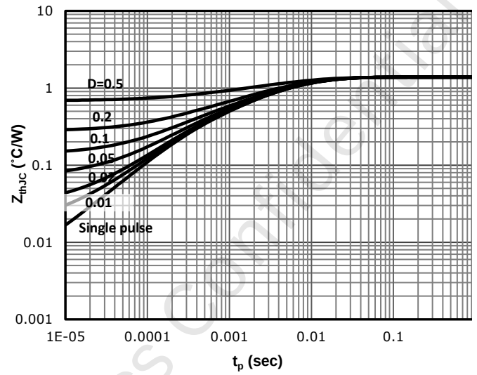
Figure 8. Transient Thermal Impedance (Junction - Case)
