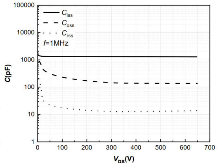
Fig 12: Capacitance Characteristics
