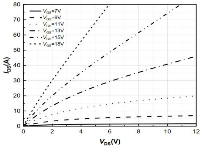
Fig 3: Output Characteristics
