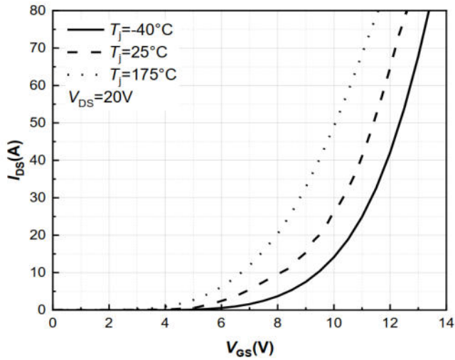
Fig 7: Transfer Characteristics
