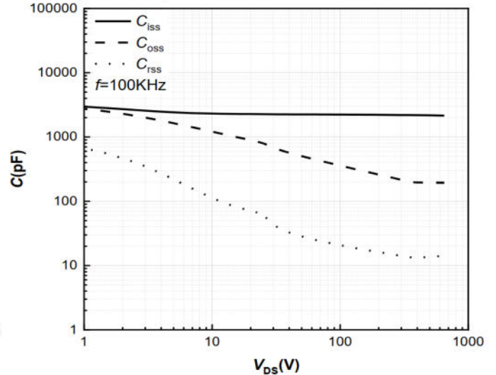
Fig 12: Capacitance Characteristics
