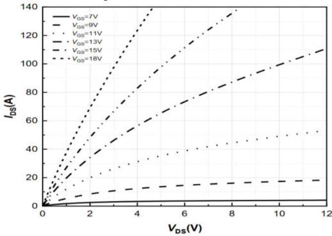
Fig 3: Output Characteristics
