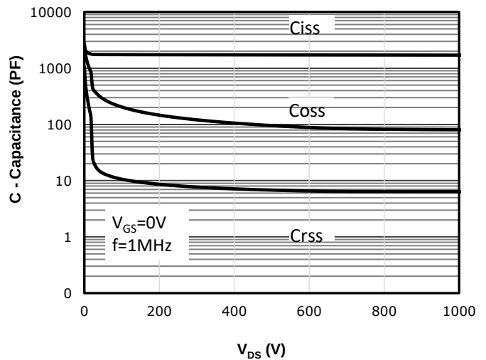
Fig 12: Capacitance Characteristics
