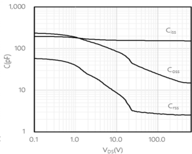
Fig 12: Capacitance Characteristics
