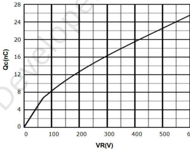
Figure 7. Total capacitance charge vs. reverse voltage
