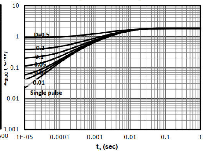
Figure 8. Transient Thermal Impedance (Junction - Case)
