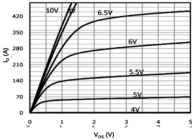
Fig 1: Output Characteristics
