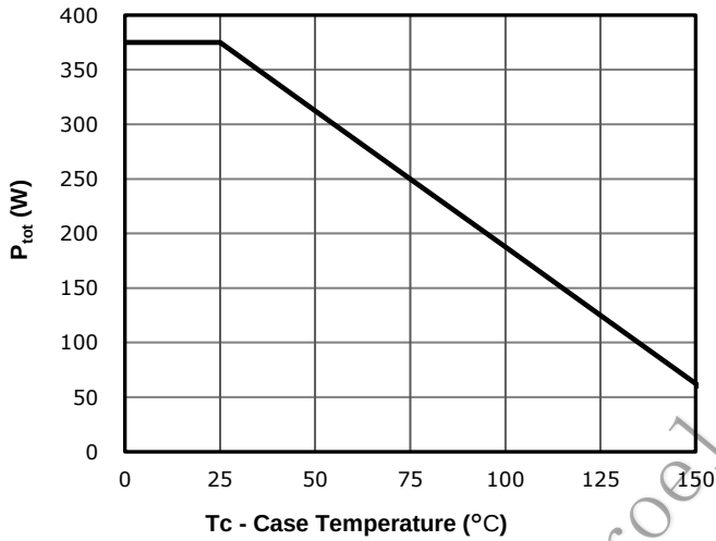
Fig 9: Power Dissipation
