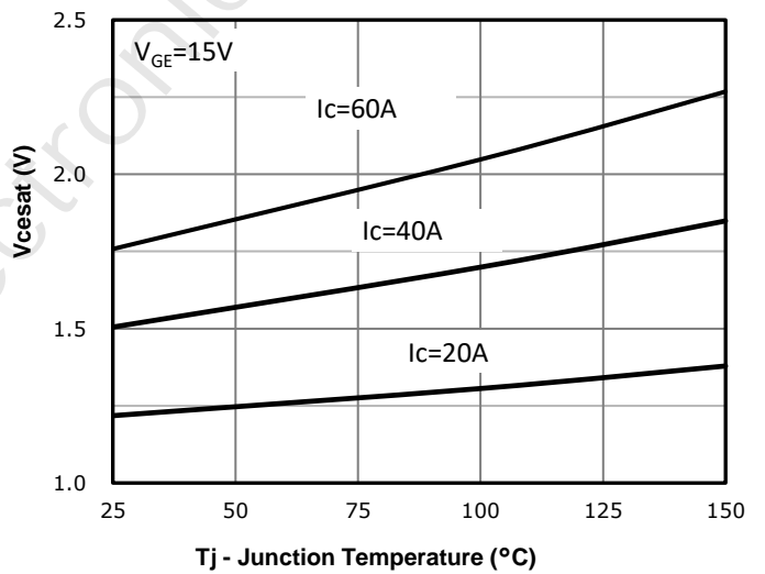
Fig 4: Typical collector-emitter voltage
