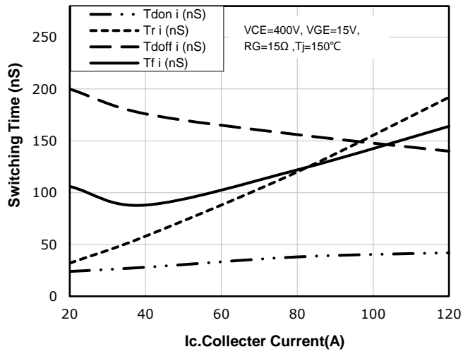
Fig 13: Typical switching times
