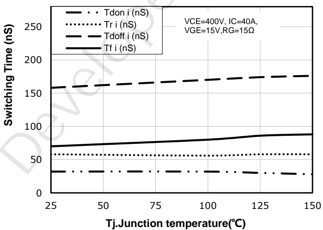
Fig 11: Typical switching times as a function of junction temperature
