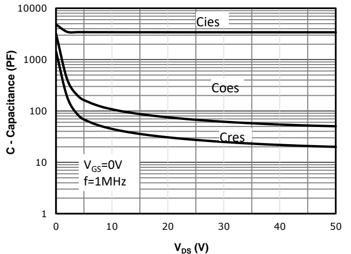
Fig 6: Capacitance Characteristics
