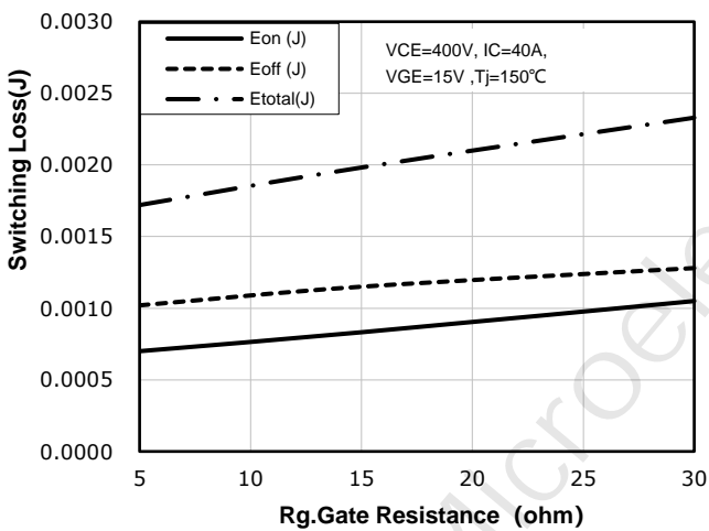
Fig 9: Typical switching energy losses as a function of gate resistor
