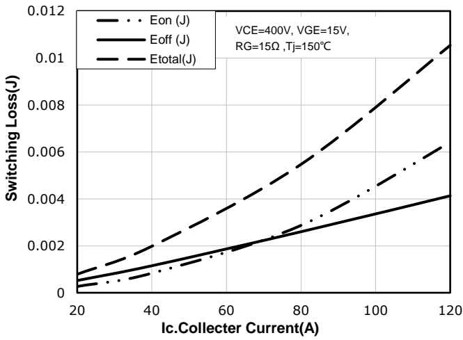
Fig 7: Typical switching energy losses
