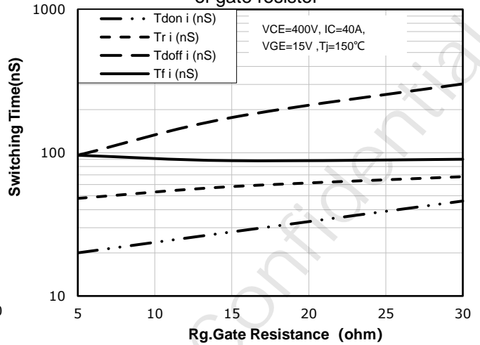
Fig 8: Typical switching times as a function of gate resistor
