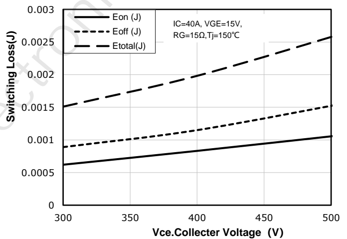
Fig 10: Typical switching energy losses as a function of collector emitter voltage
